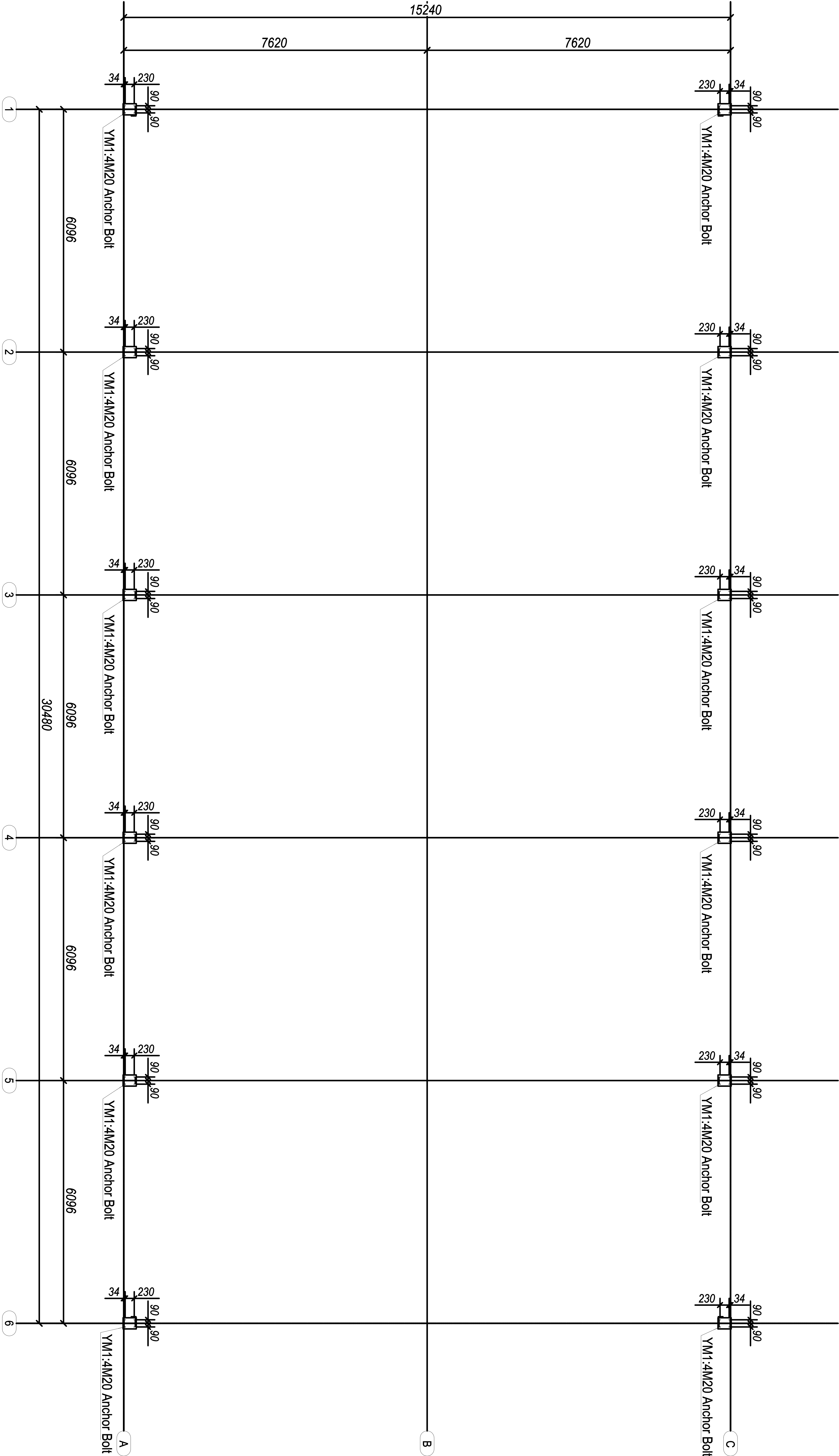
Buiding7B Achor bolt layout plan
