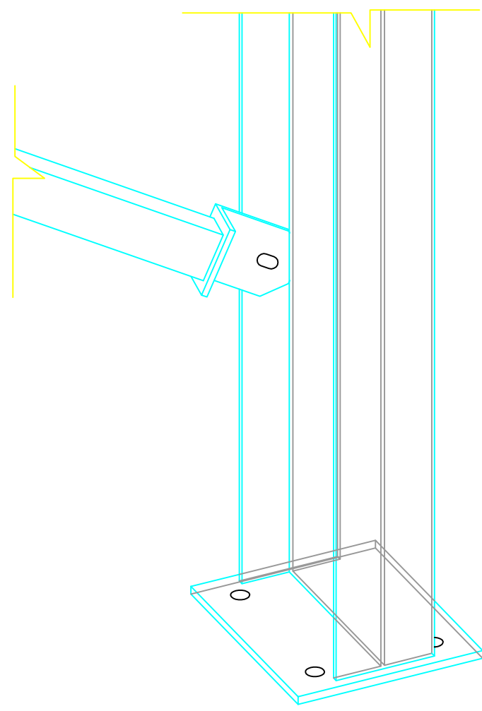
Wind brace joint detail
