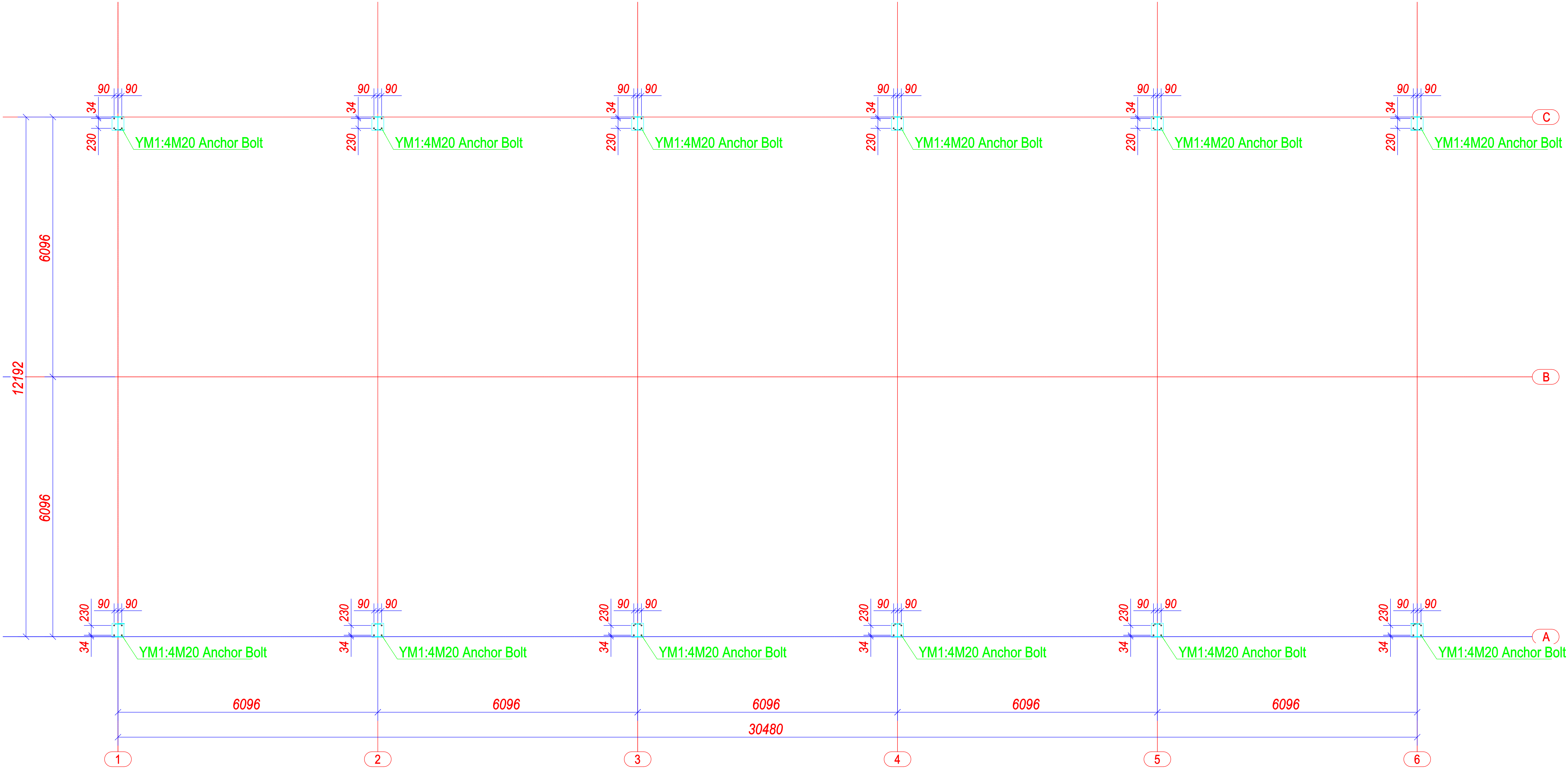
Buiding6B chor bolt layout plan
